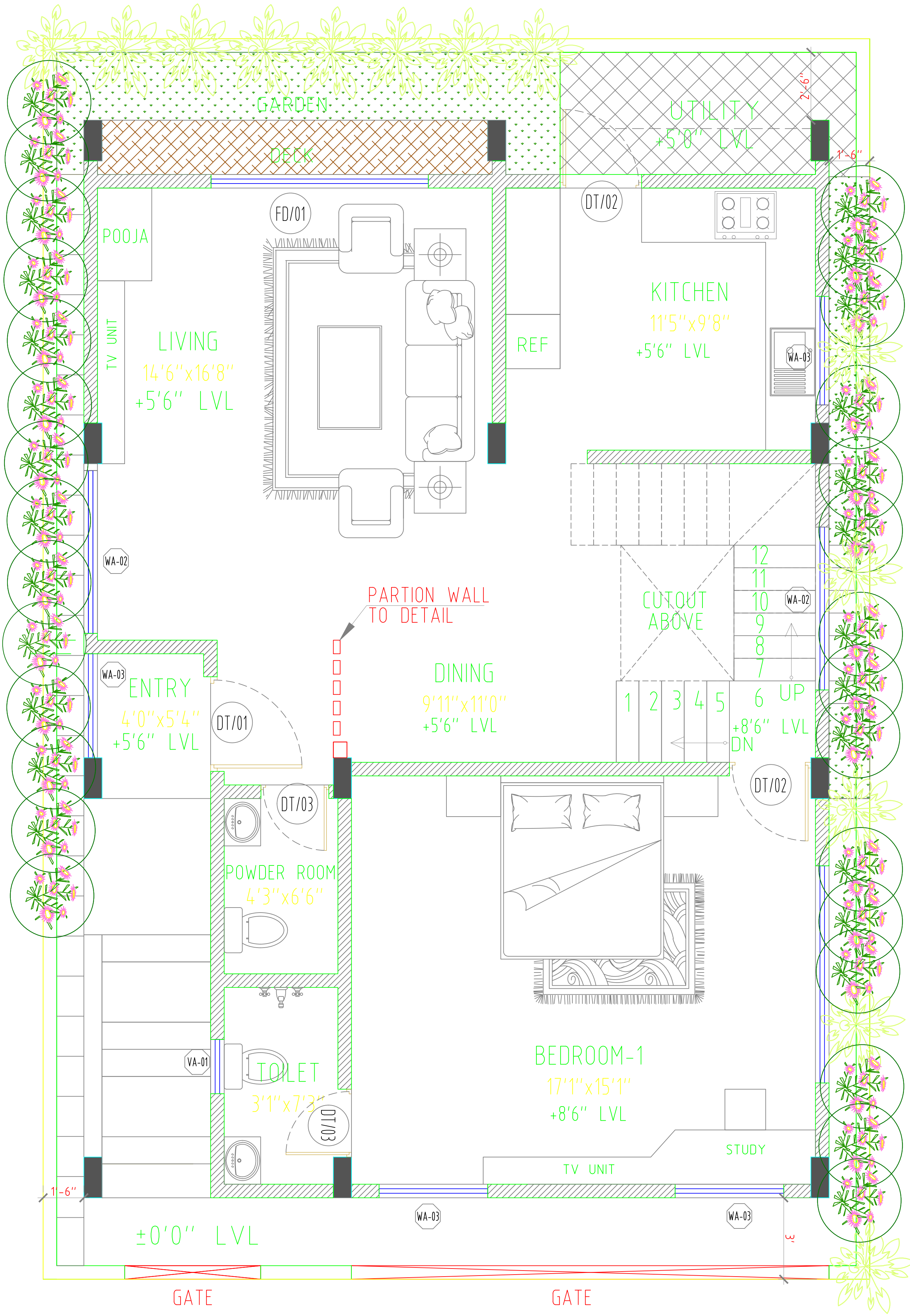
GROUND FLOOR PLAN - LEVEL 1 01
